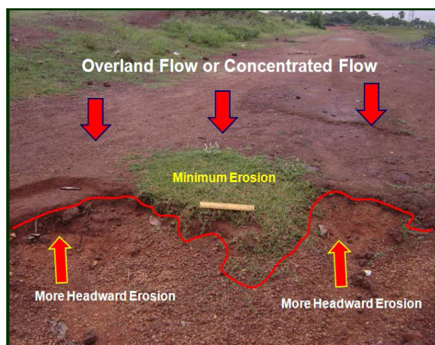
Figure 6: Shows the vegetal cover to protect the headward erosion during concentrated flow.
